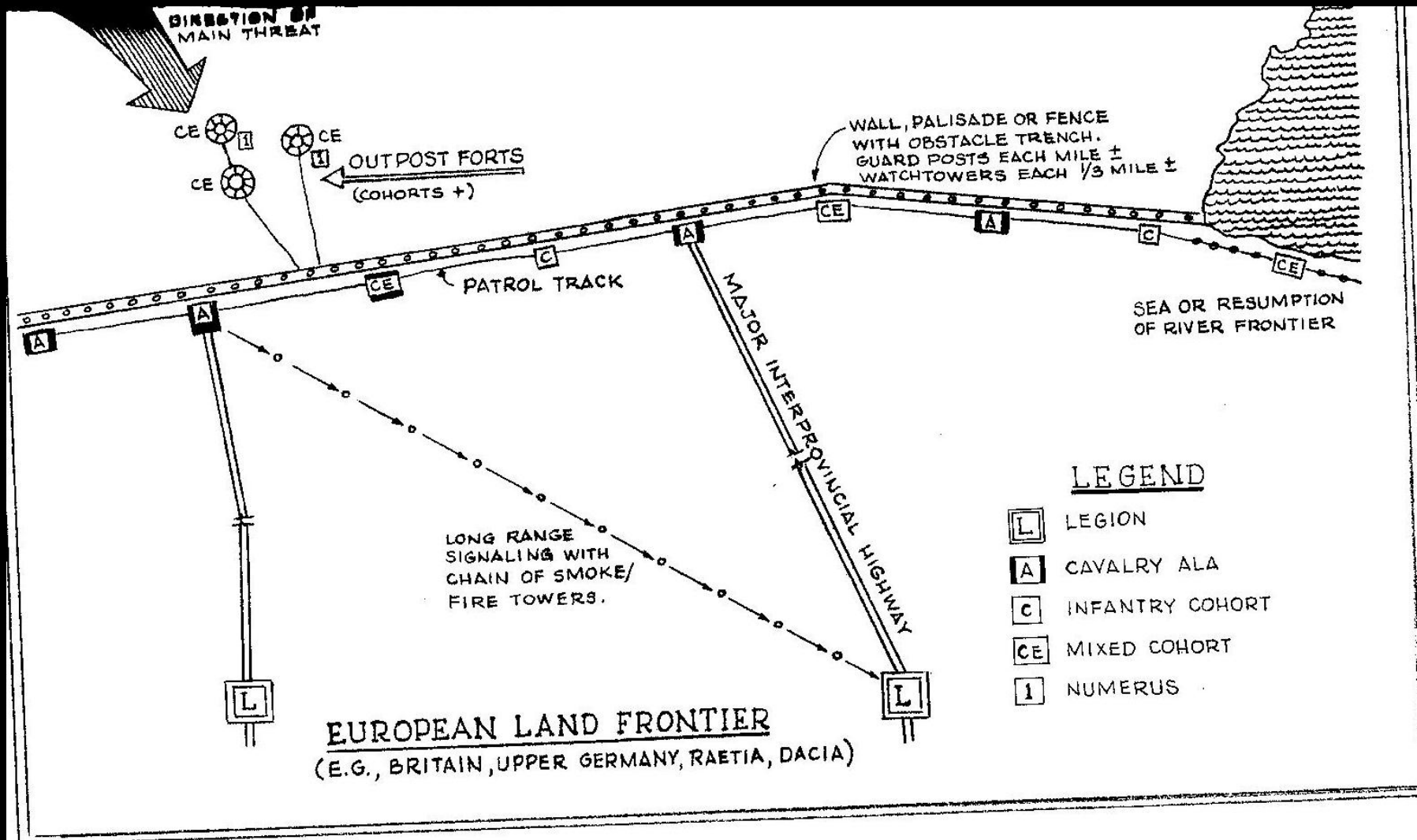
FIG. 2.2. MODELS OF FRONTIER ORGANIZATION II
